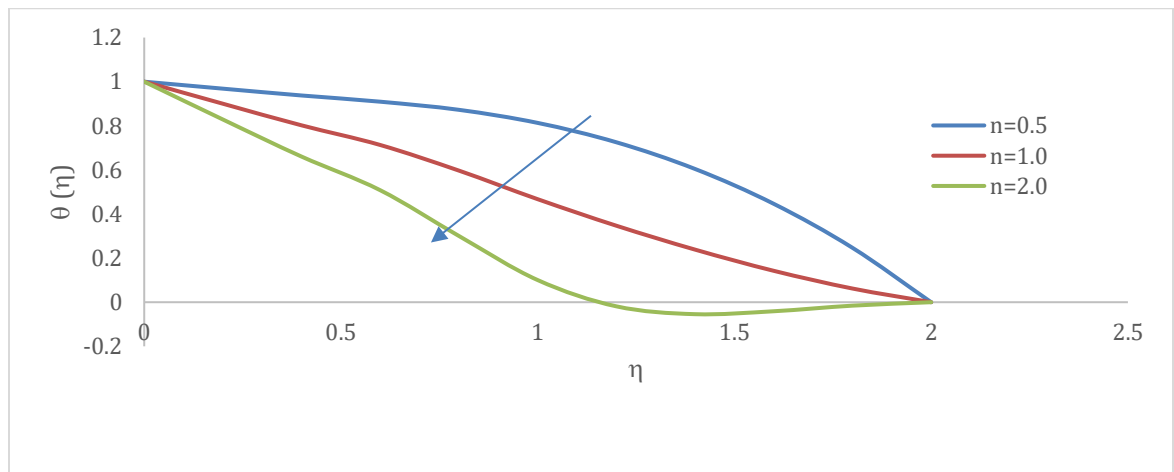
Figure 8. Varying of n on temperature profiles
