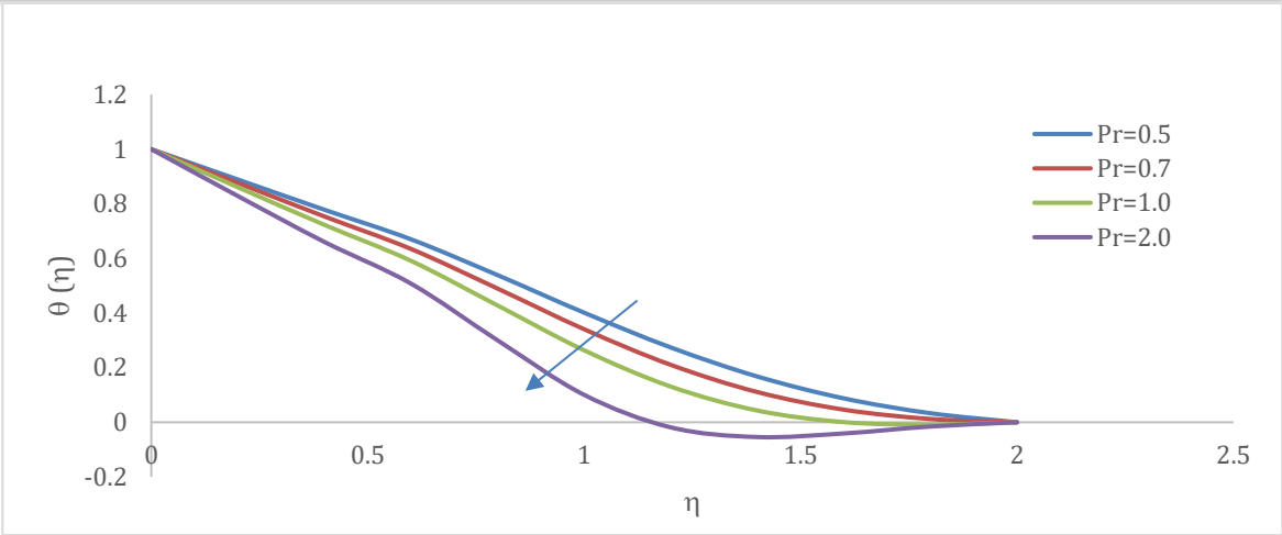
Figure 20. Varying of Pr on temperature profiles.
