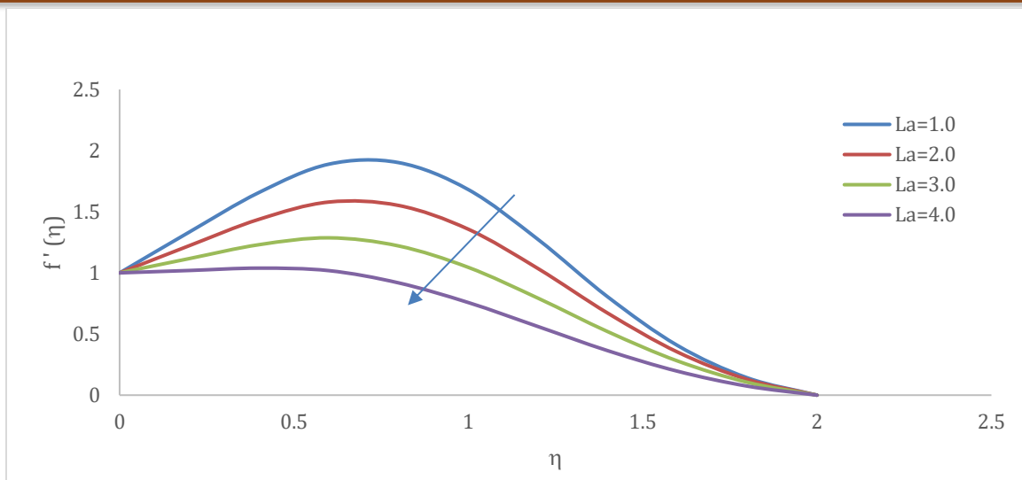
Figure 12. Varying of La on velocity profiles.
