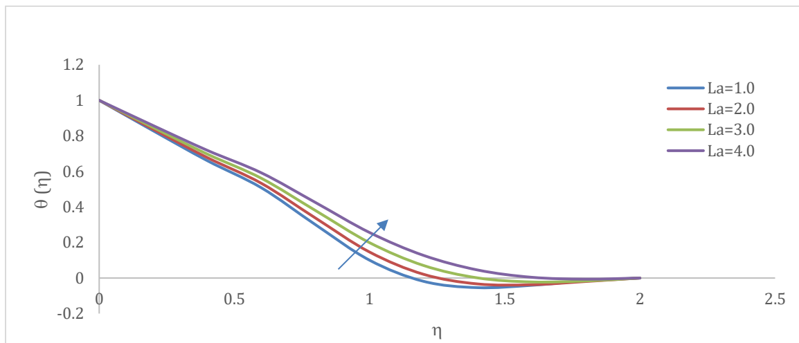
Figure 13. Varying of La on temperature profiles.
