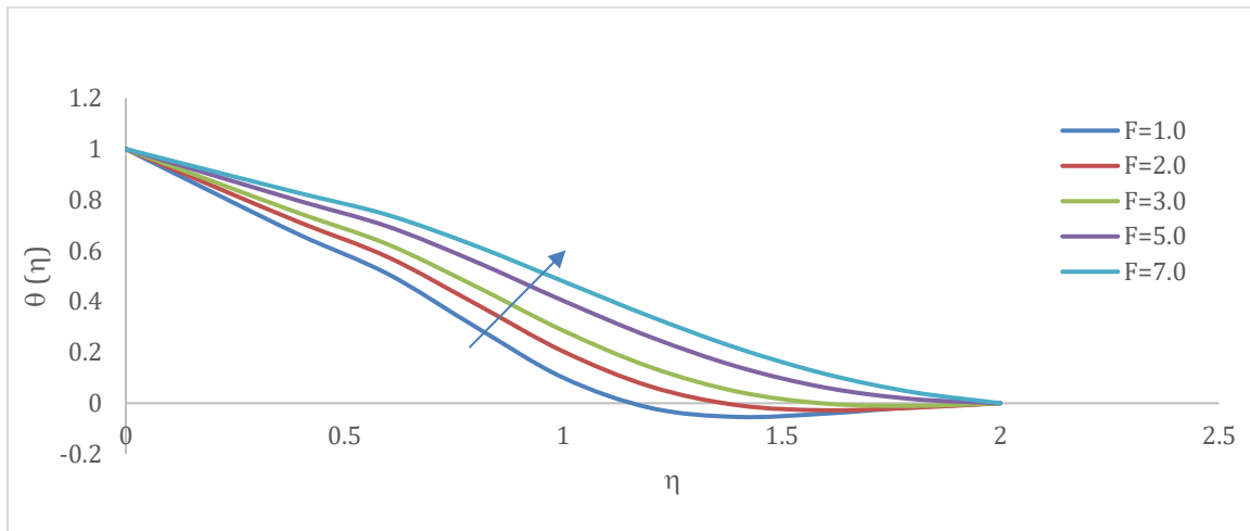
Figure 5. Varying of F on temperature profiles.
