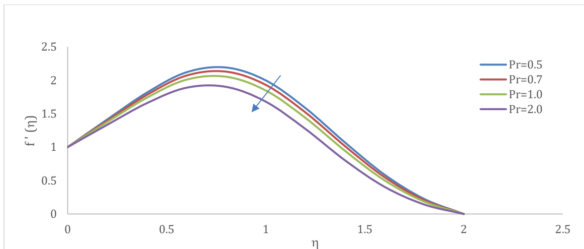
Figure 19. Varying of Pr on velocity profiles.
