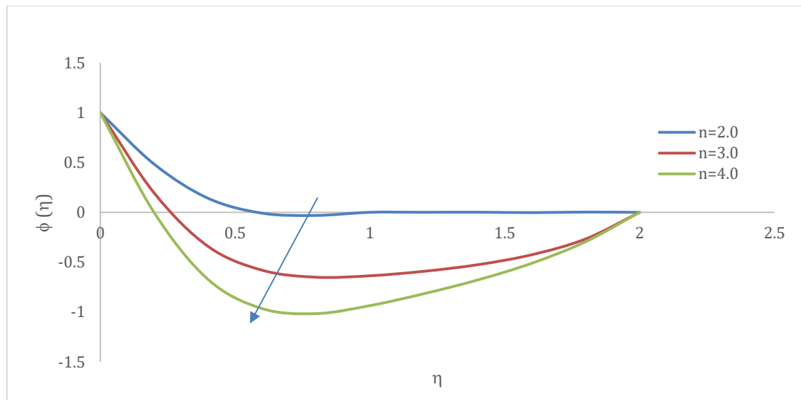
Figure 9. Varying of n on nano-particle concentration profiles
