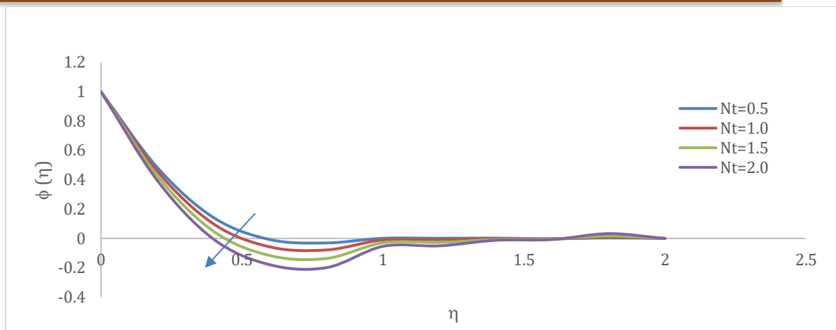
Figure 18. Varying of Nt on nano-particle concentration profiles.
