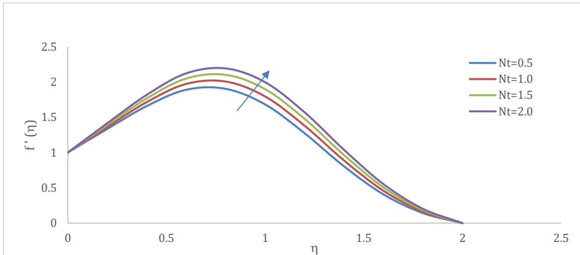
Figure 16. Varying of Nt on velocity profiles.
