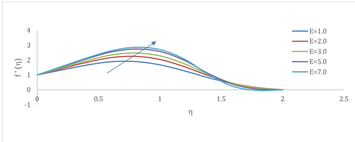
Figure 1. Varying of E on velocity profiles.
