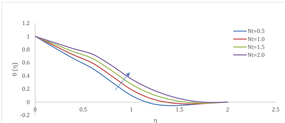
Figure 17. Varying of Nt on temperature profiles.
