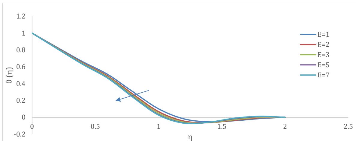
Figure. 2 Varying of E on temperature profiles.
