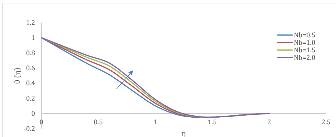
Figure 15. Varying of Nb on temperature profiles.
