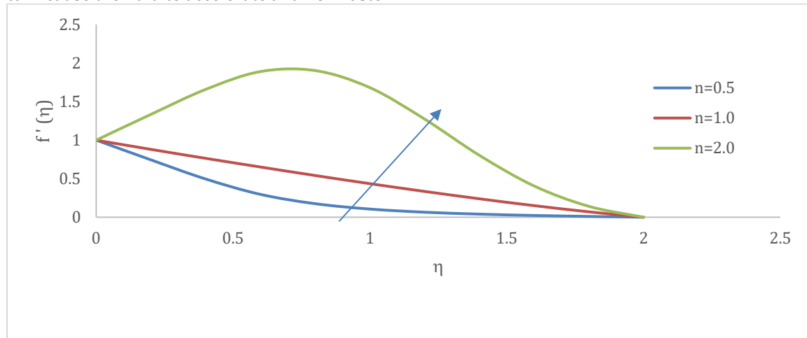
Figure 7. Varying of n on Velocity profiles.
