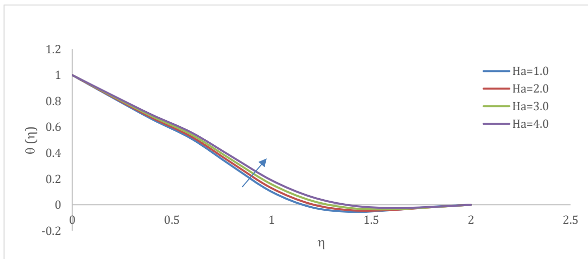
Figure 11. Varying of Ha on temperature profiles.
